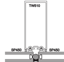
④ VERTICAL MULLION
