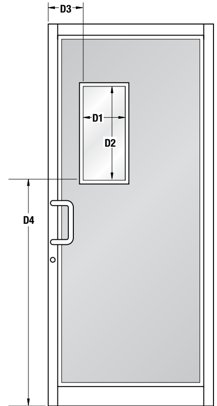
Series 1000 Flush Panel 250 Narrow Stile Offset Hung (Exterior View)
